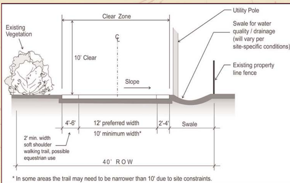
Trolley Trail conceptual design
